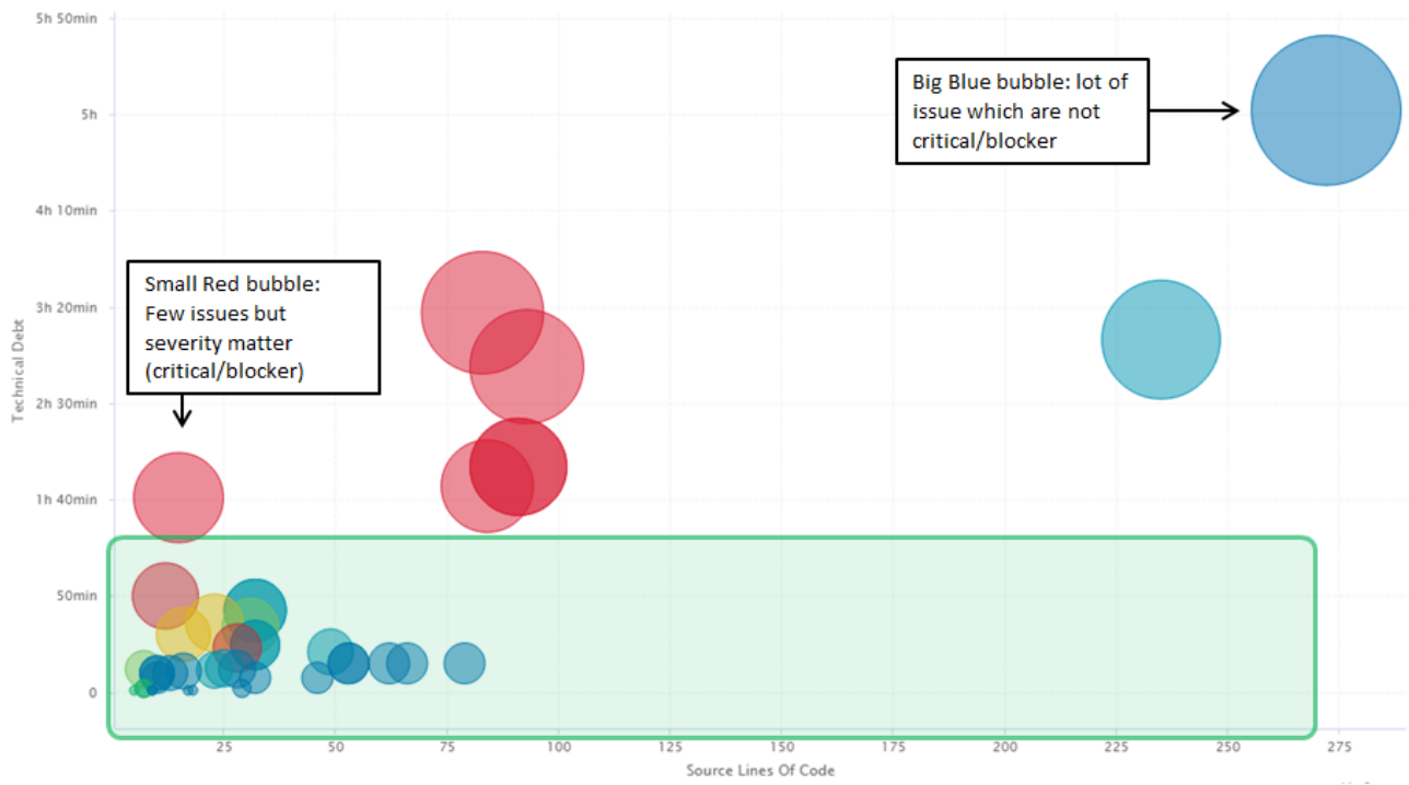
Technical Debt - Module distribution
