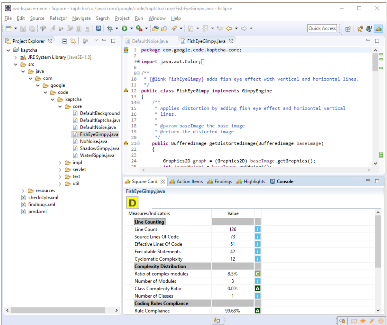
The Squore Perspective with the Squore Card, Action items, Findings and Highlights views in the bottom panel
