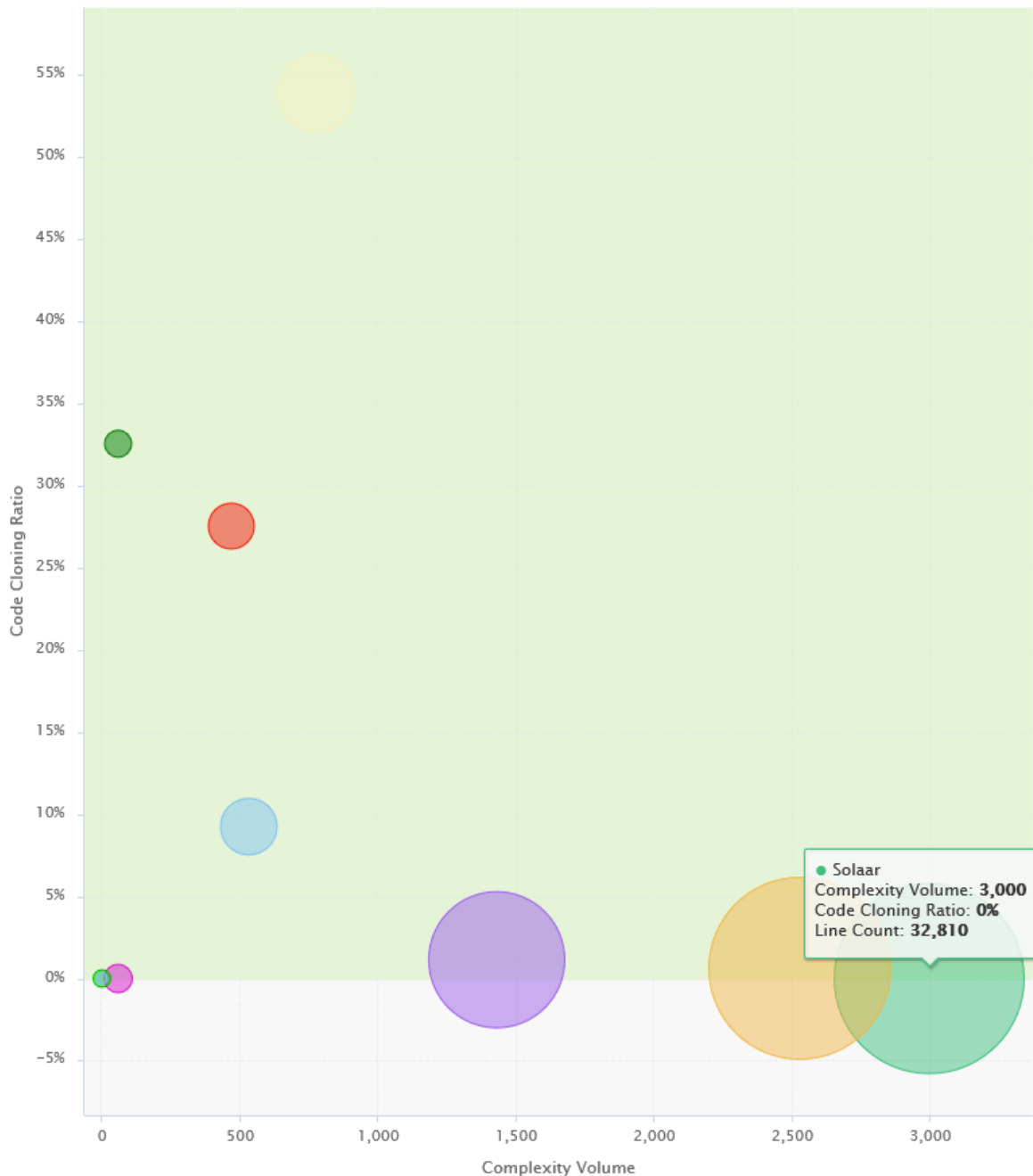
Complexity Volume Vs Cloning for current Software Analytics projects
