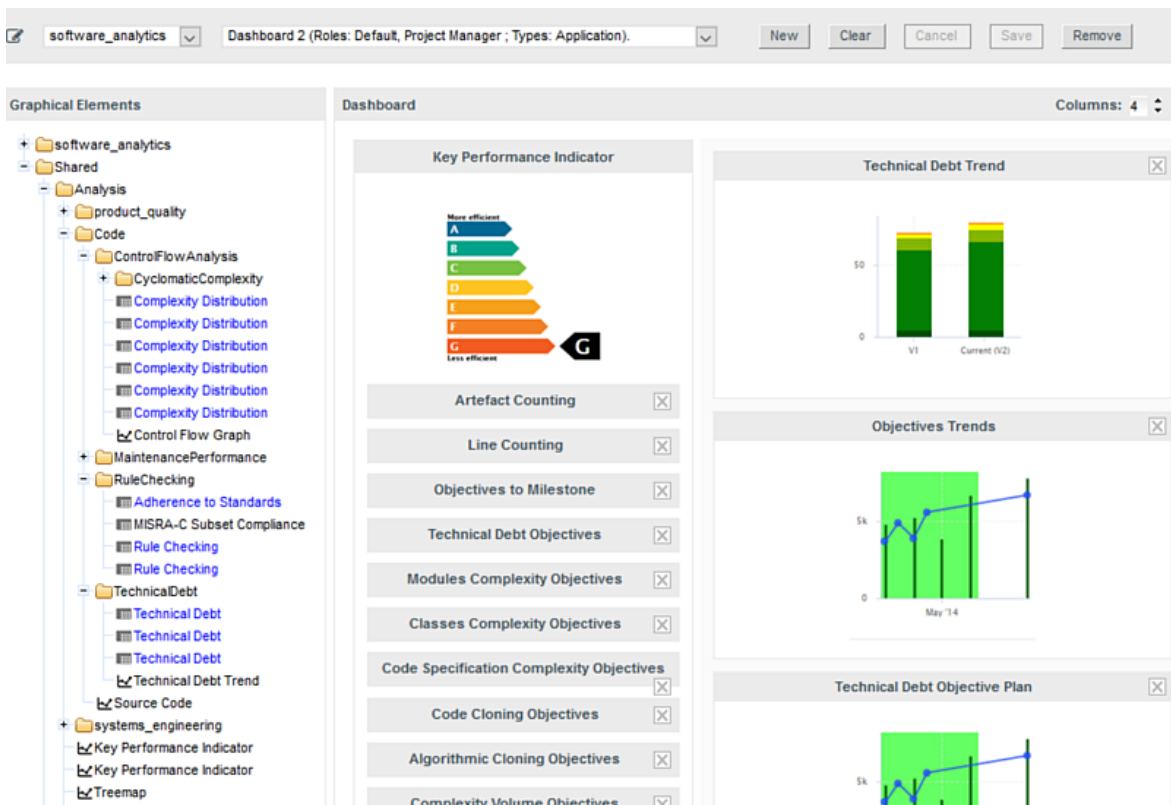
The Software Analytics model in the Dashboard Editor
