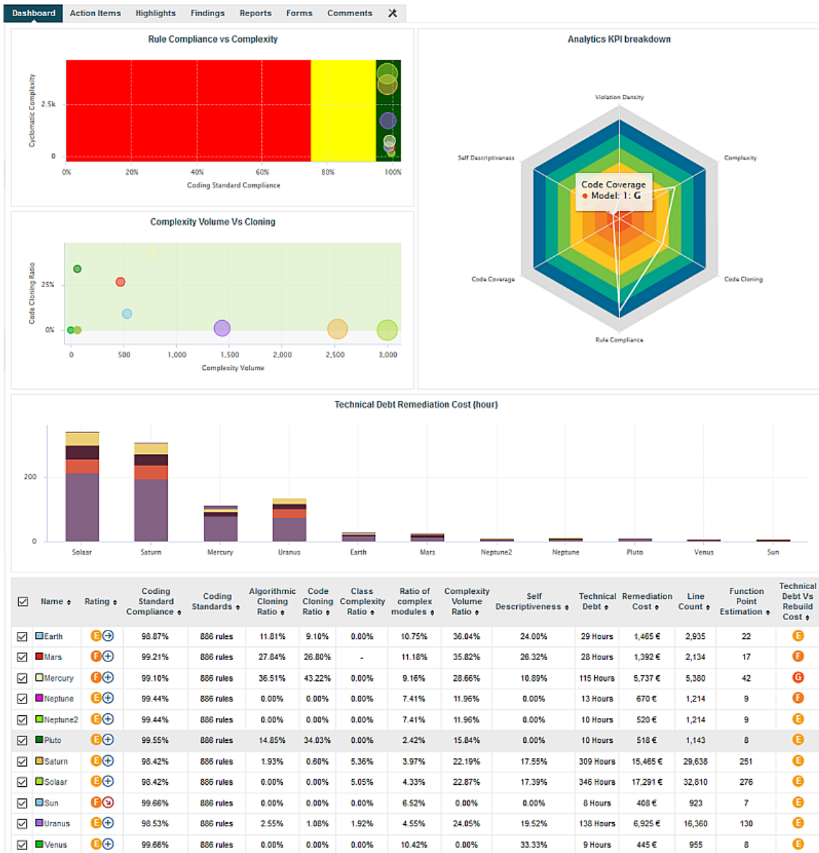
The analysis model dashboard for Software Analytics projects
