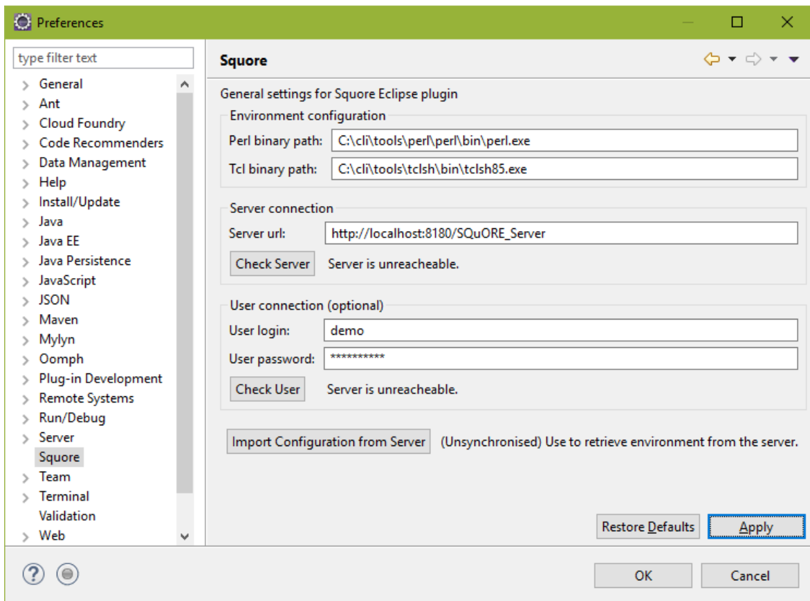
The Squore Eclipse Plugin preferences page
