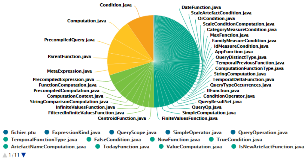
Artefact Pie
