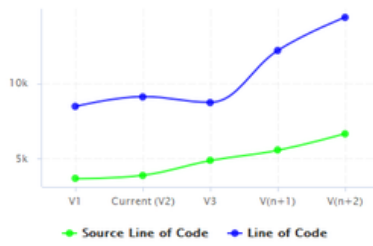
STACKED_SPLINE
