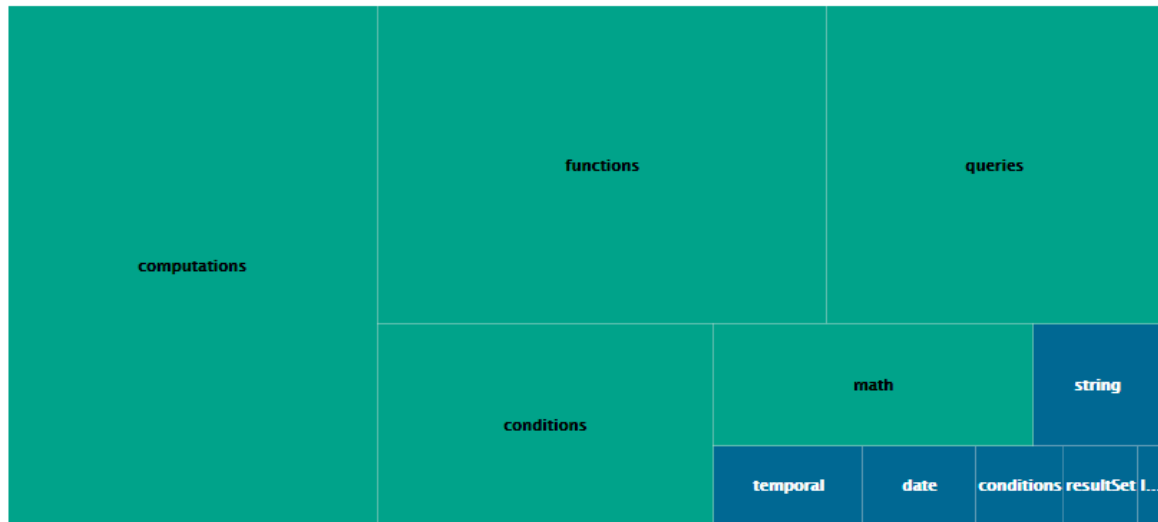
Treemap
