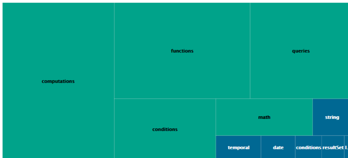
Treemap
