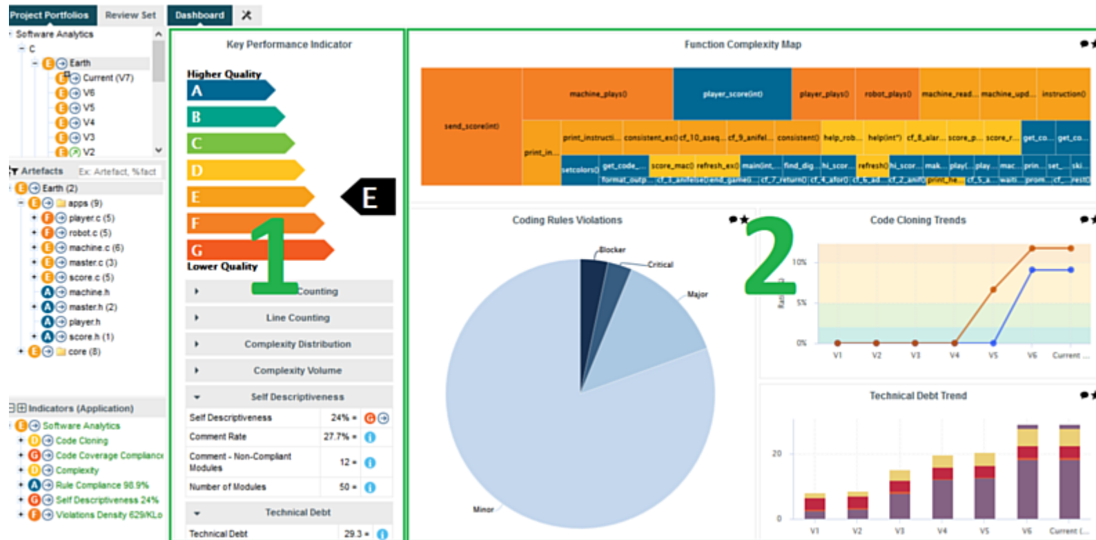
The Squore Artifact Dashboard Areas
