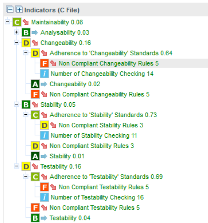
The Indicator Tree for player.c
